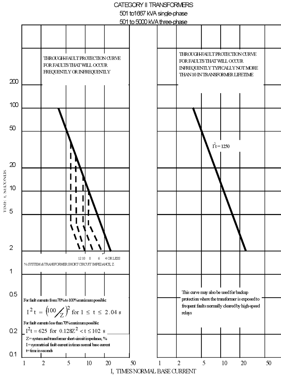
Figure 2—Category II transformers
