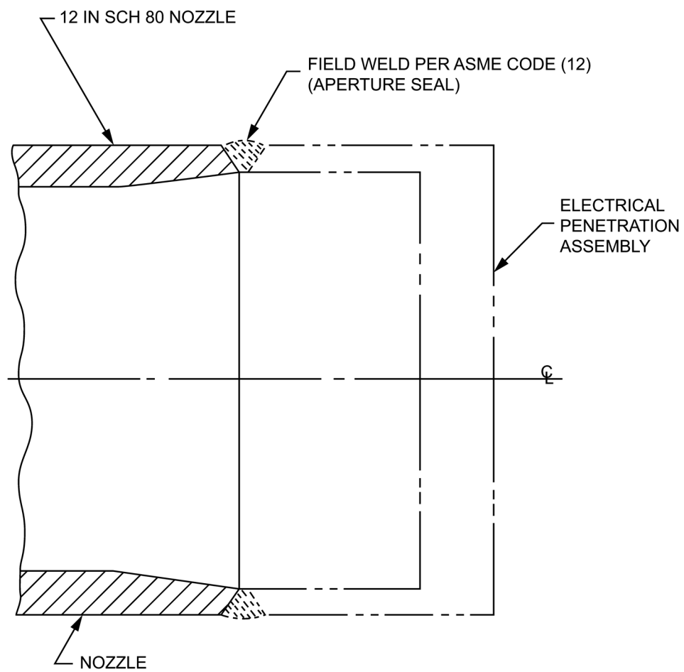
Figure B.1—Weld-in interface
