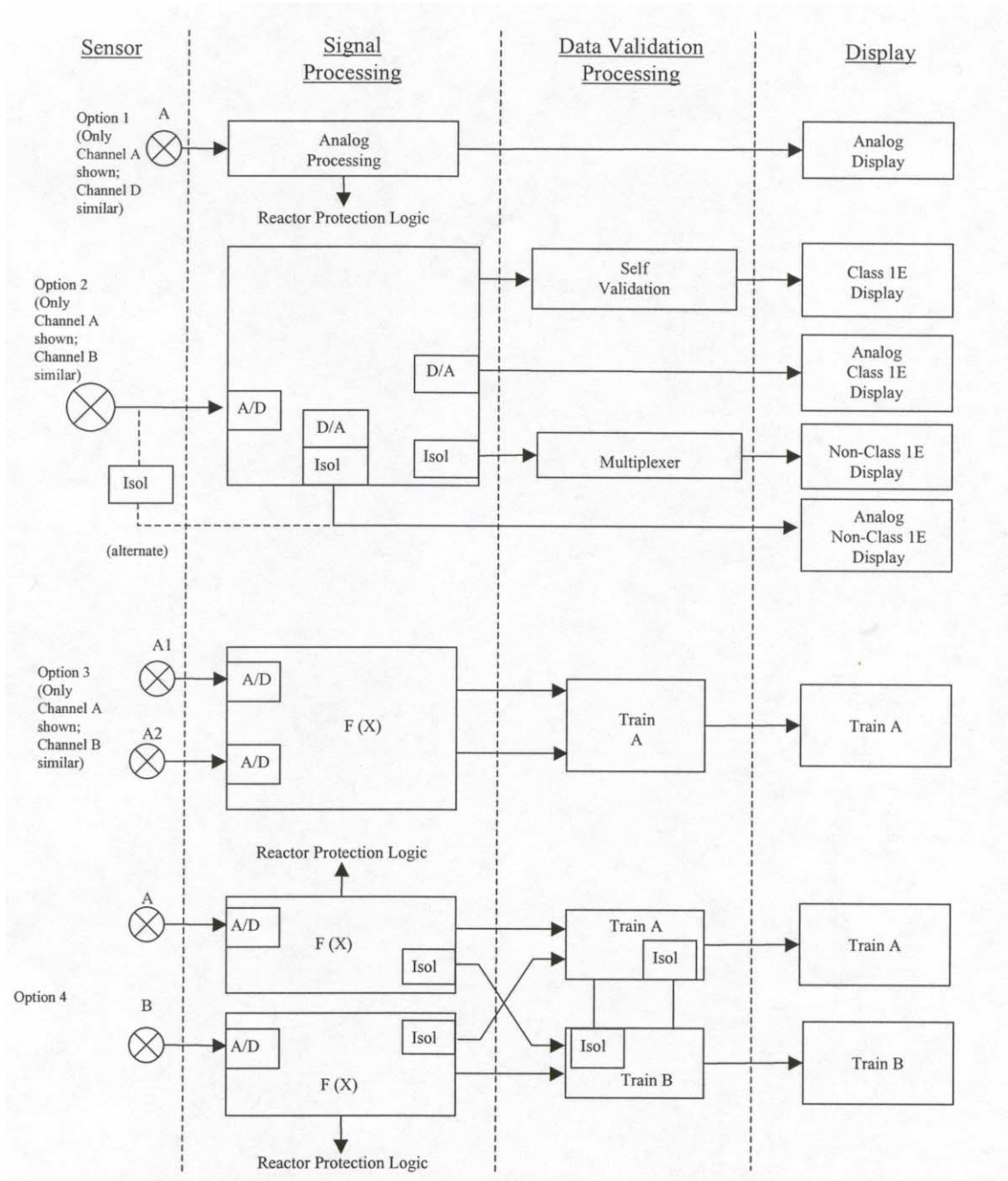
Figure 2—Examples of monitoring channel displays
