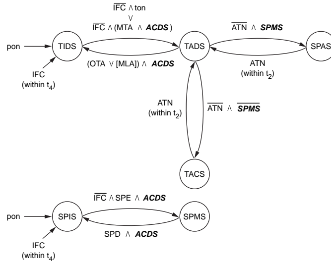
Figure 5—AH state diagram
